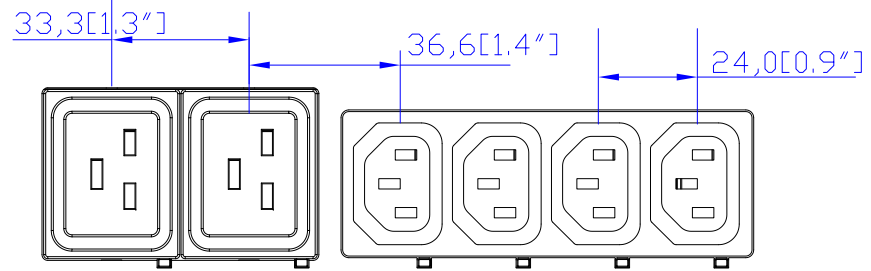
VIEW B
