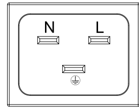
IEC320 C20
